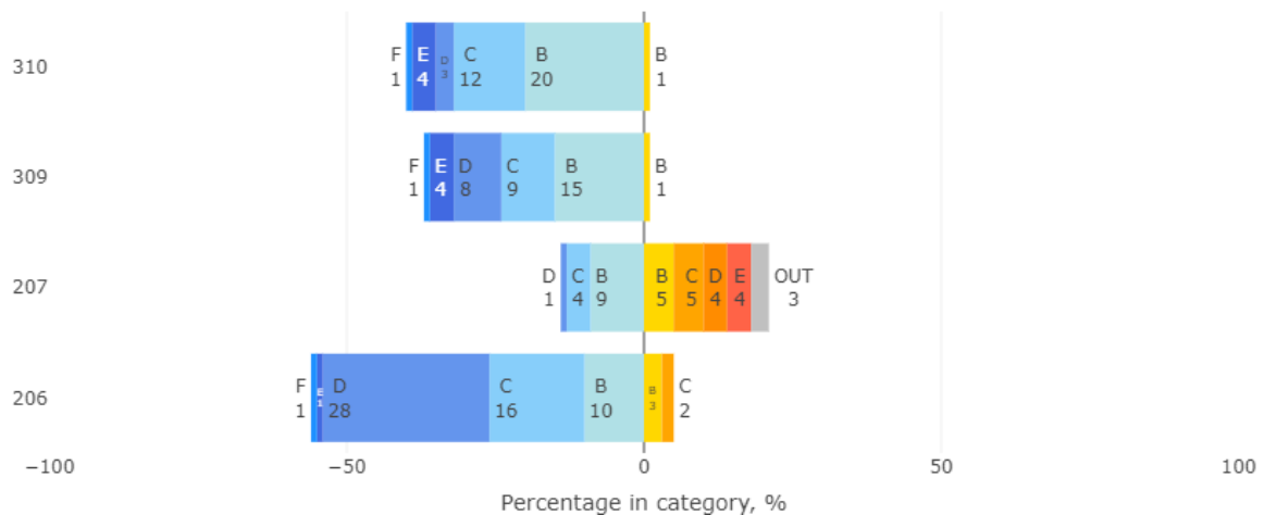
Figure 36. Temperatures spent in each category other than category A indicating the hot and cold limits (full period of data)
