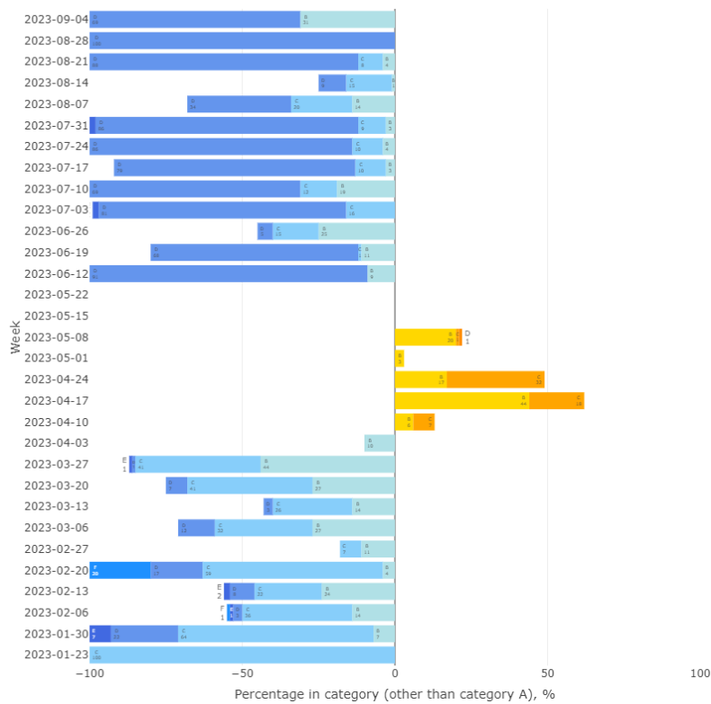
Figure 107. Temperatures spent in each category other than category A indicating the hot and cold limits (weekly)
