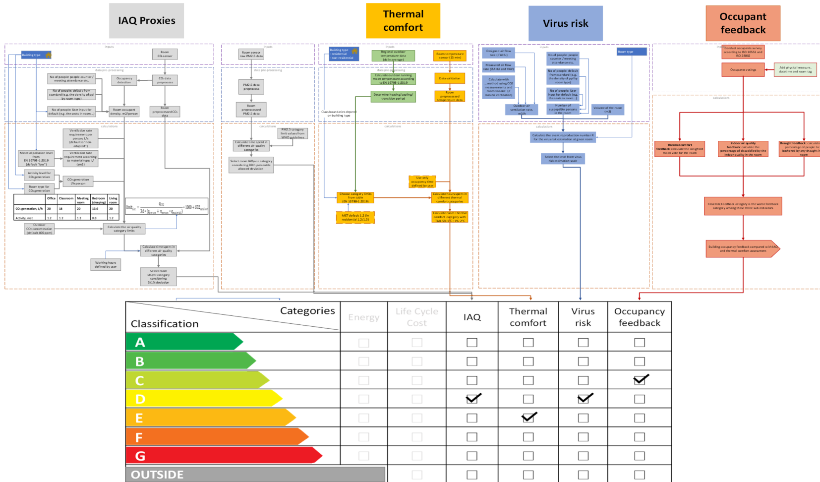
Figure 1: The framework of the IEQ assessment methodology
