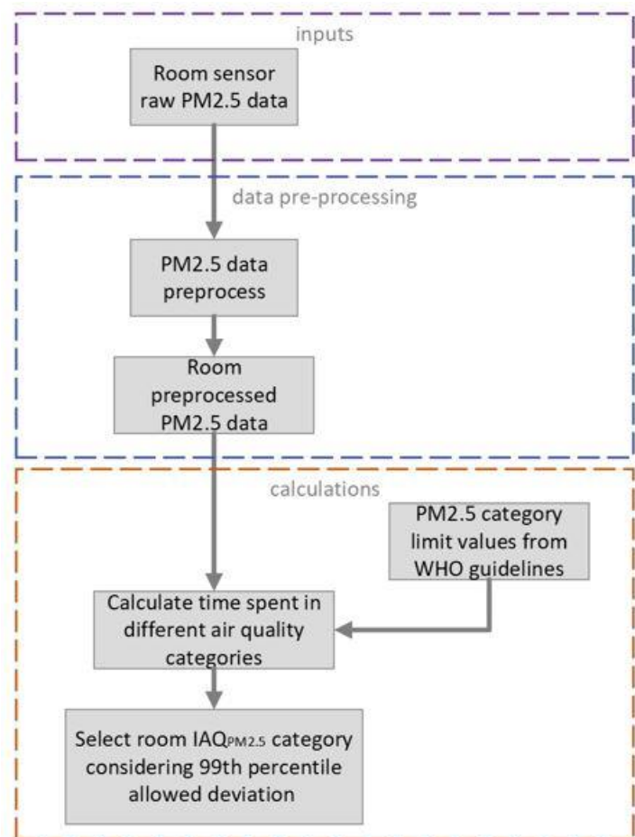
Figure 10: PM2.5 level based IAQ assessment procedure for a single room
