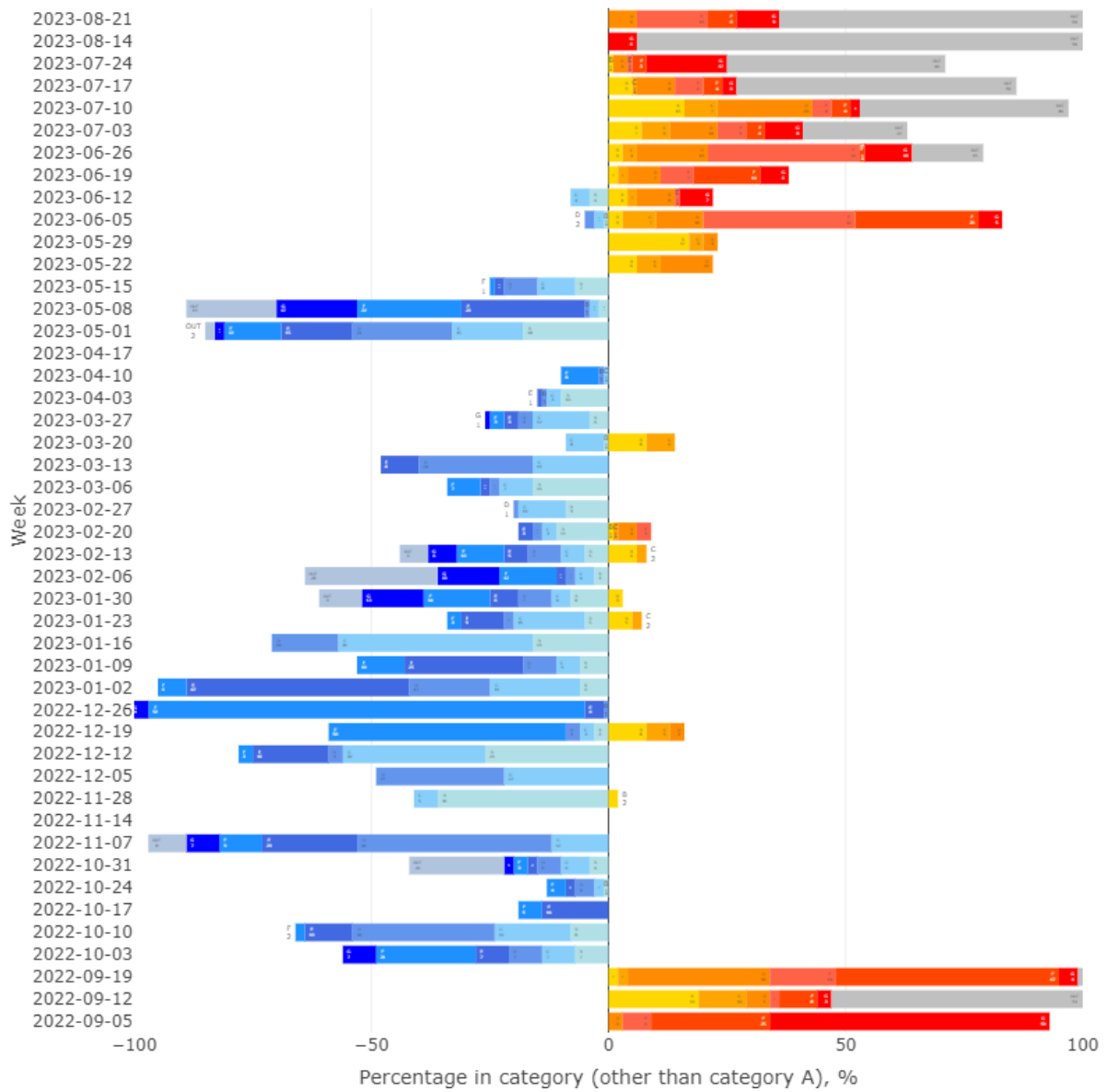
Figure 21. Temperatures spent in each category other than category A indicating the hot and cold limits (weekly)
