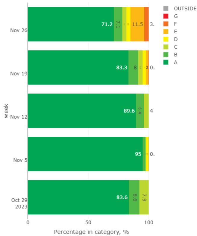
Figure 104. Measured CO2 concentration – percentage of time spent in each category (weekly)
