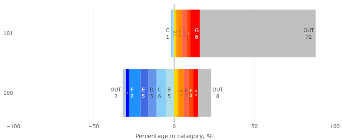
Figure 18. Temperatures spent in each category other than category A indicating the hot and cold limits (full period of data)
