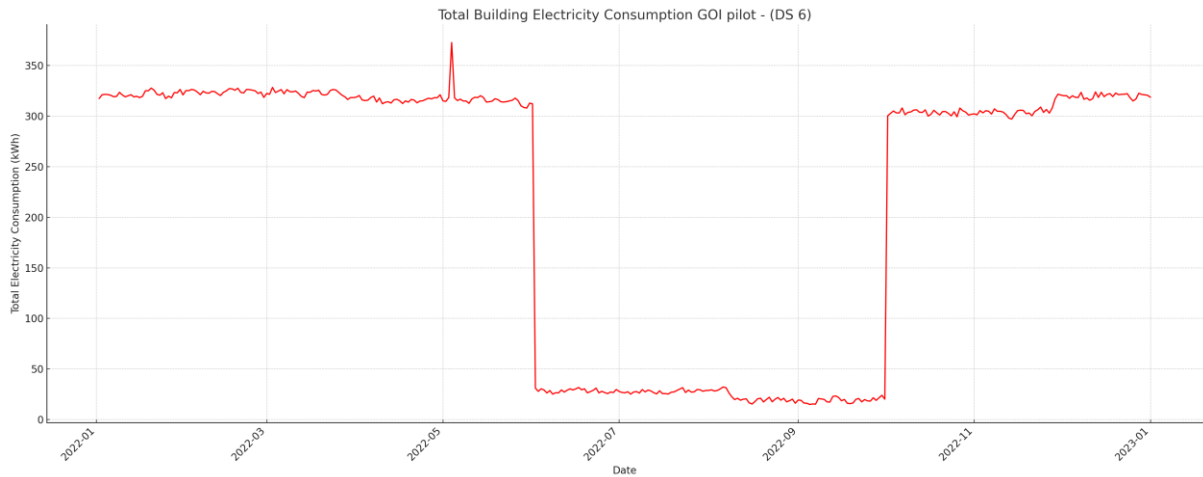
Figure 61 - Total Building electricity consumption DS6 pilot
