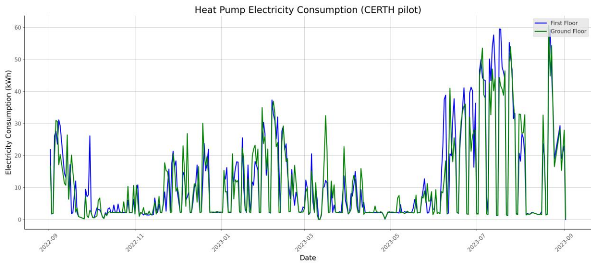
Figure 58 - Heat pump electricity consumption CERTH pilot
