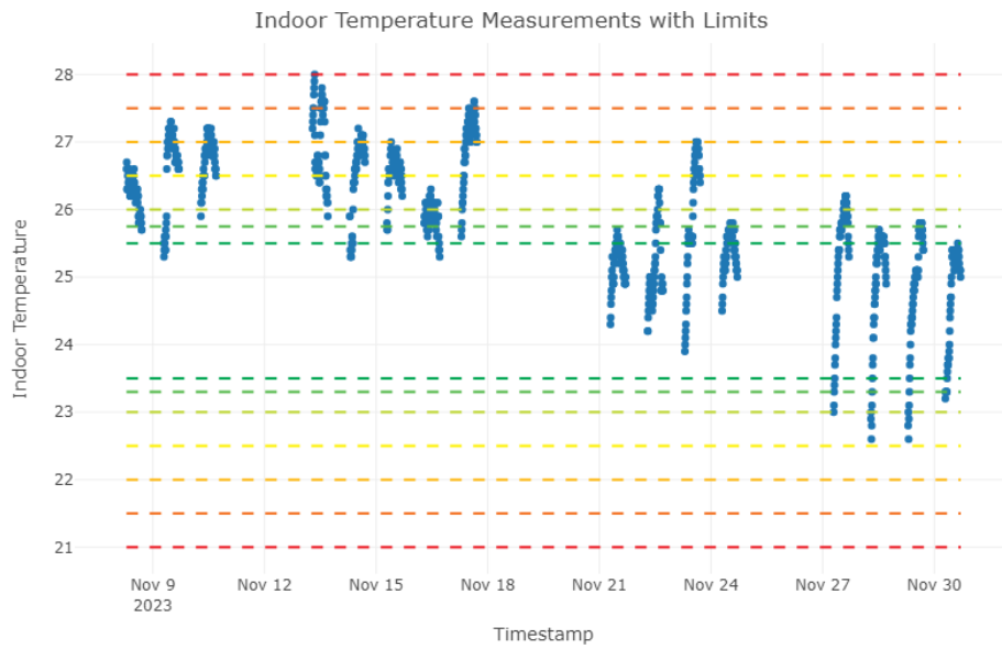
Figure 30. Temperature measurement and limits in cafeteria (number 101) (with only upper limits in summer and lower limits in winter season)
