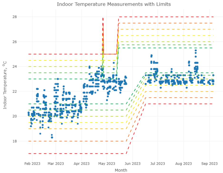
Figure 105. Temperature measurement and limits in meeting room (number 206)
