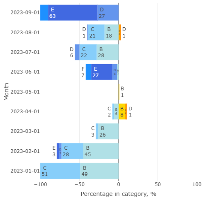
Figure 114. Temperatures spent in each category other than category A in room 310 indicating the hot and cold limits (monthly)
