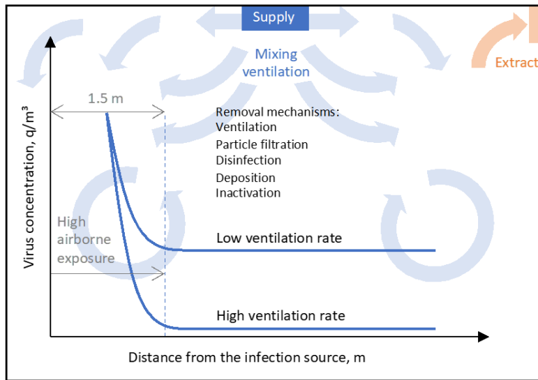
Figure 15: Main removal mechanisms of virus-containing particles
