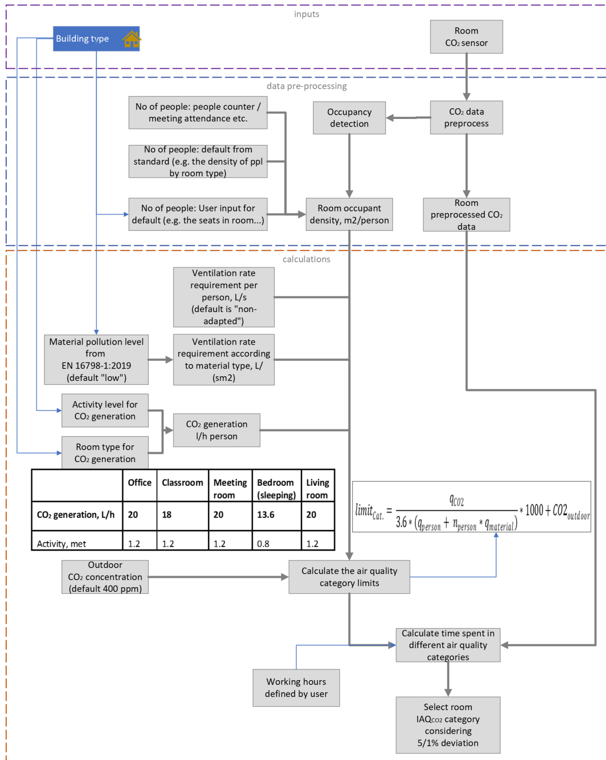
Figure 6: CO 2 level based IAQ assessment procedure for a single room
