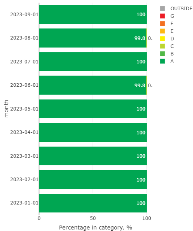
Figure 116. Measured CO2 concentration – percentage of time spent in each category (monthly)
