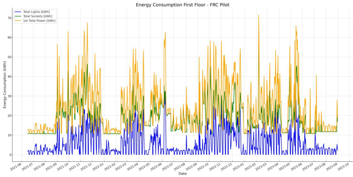
Figure 56 - Energy consumption first floor FRC pilot
