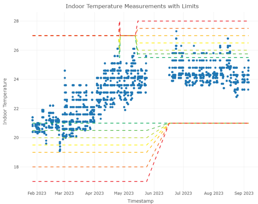
Figure 38. Temperature measurement and limits in office (number 207) (with only upper limits in summer and lower limits in winter season)
