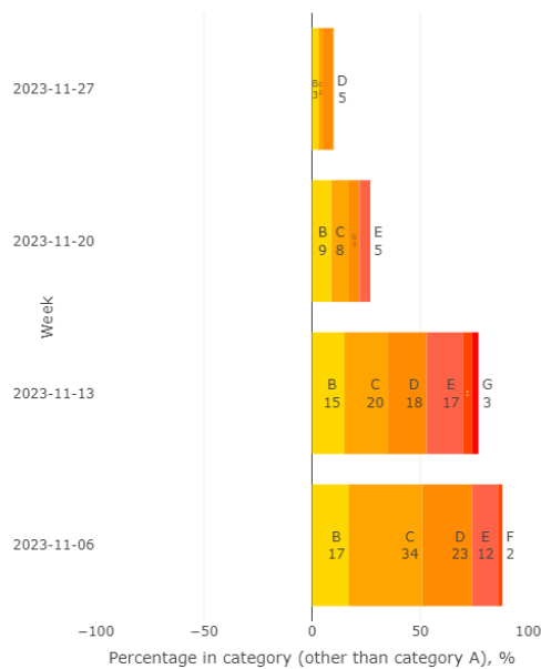
Figure 97. Temperatures spent in each category other than category A in room 207 indicating the hot and cold limits (weekly)
