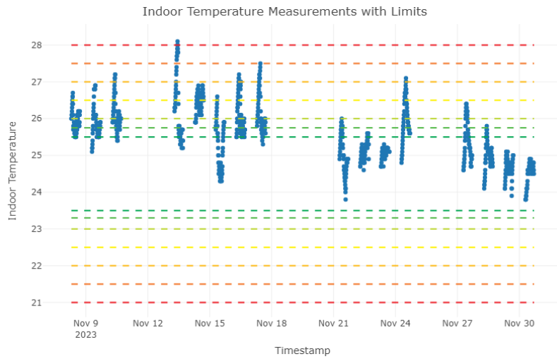
Figure 95. Temperature measurement and limits in classroom (number 207)
