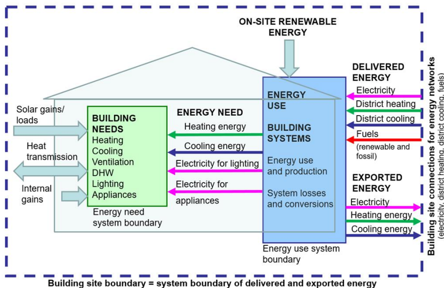
Figure 50: System boundaries for energy need, energy use, delivered energy, exported energy, and on-site generated renewable energy [26]
