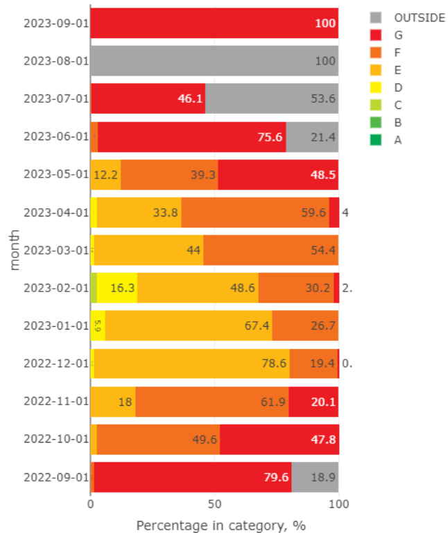
Figure 23. Measured CO2 concentration – percentage of time spent in each category (monthly)
