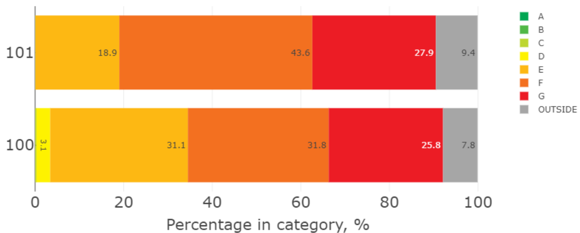
Figure 22. Measured CO 2 concentration – percentage of time spent in each category (full period of data)
