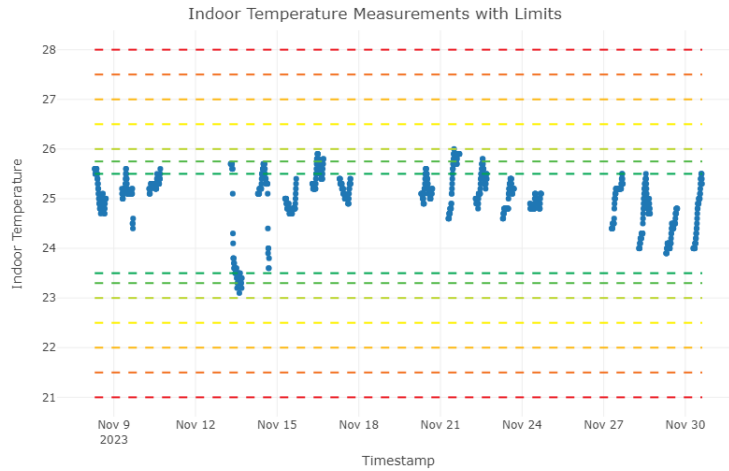
Figure 100. Temperature measurement and limits in meeting room (number 122)
