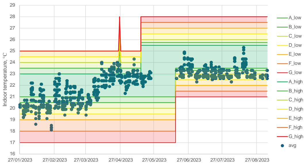
Figure 4. Indoor temperature and category limits
