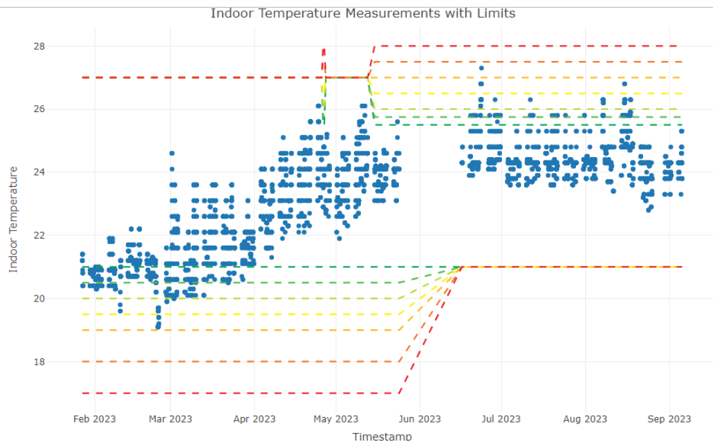
Figure 5. The indoor temperature and modified category limits (counting only too hot in summer and too cold in winter)
