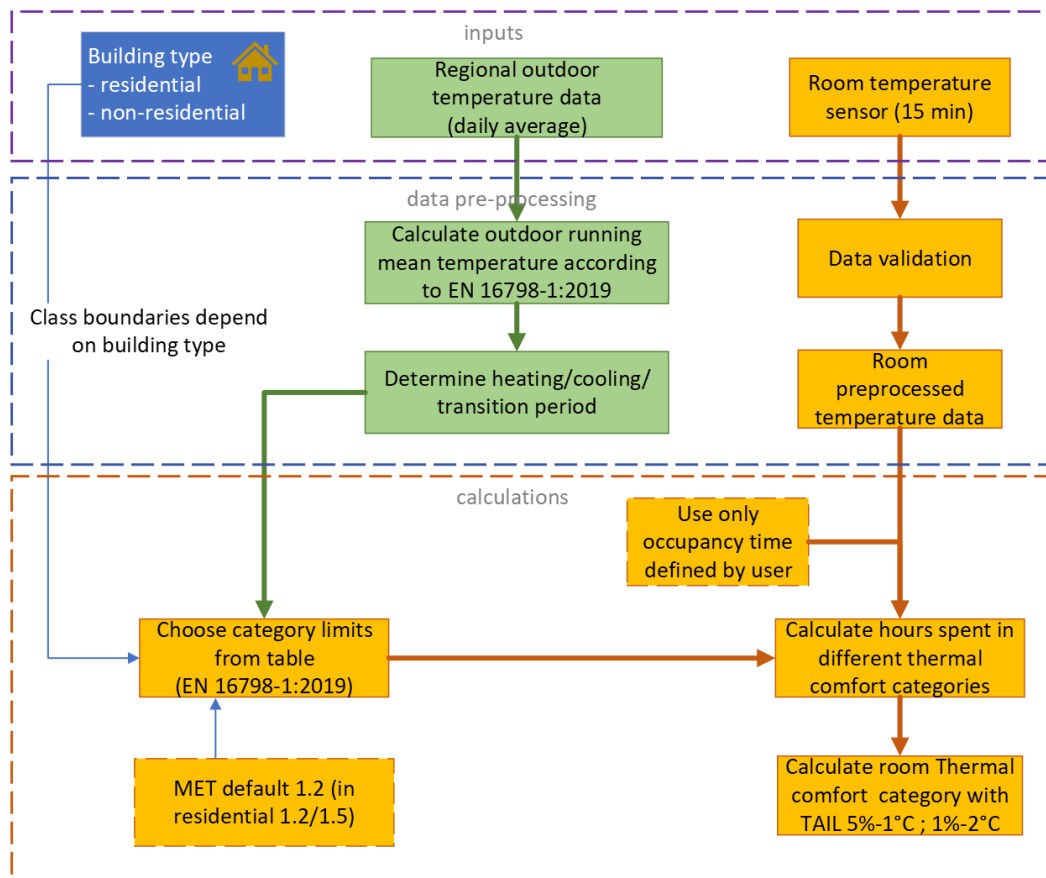
Figure 2: Procedure for computing the Thermal Comfort category according to EN 16798-1:2019
