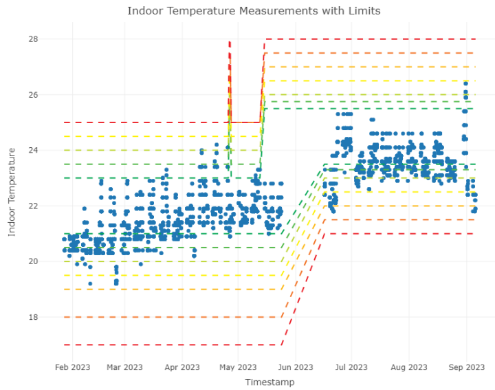
Figure 113. Temperature measurement and limits in classroom (number 310)
