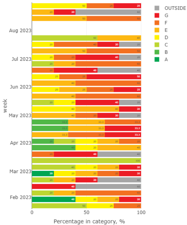
Figure 28. Measured CO2 concentration – percentage of time spent in each category (weekly)
