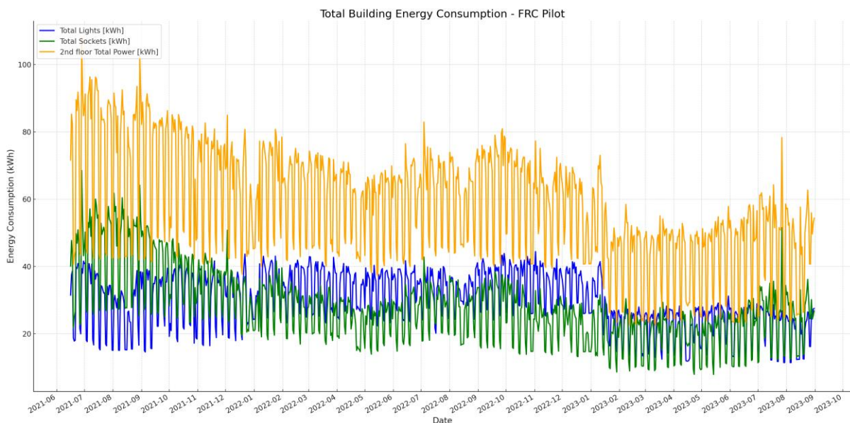
Figure 55 - Total Building energy consumption FRC pilot
